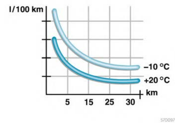
Figure 1. Fuel consumption per 100 kilometers at two different ambient temperatures.
