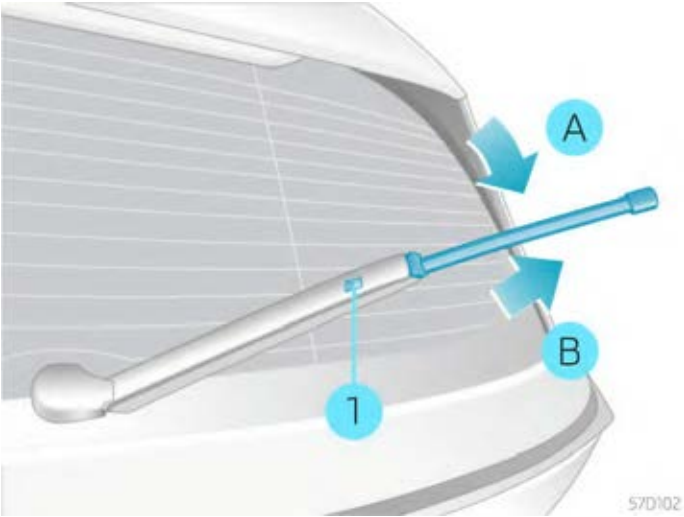
Figure 1. Replacement of rear windshield wiper blades
