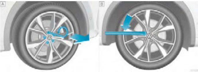
Figure 1 A. Remove the cover from the wheel bolts B. Loosen the wheel bolts
