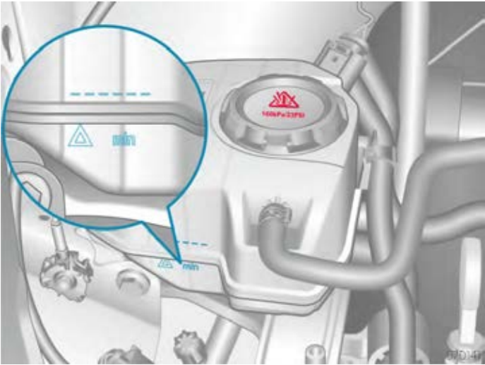
Figure 1. Liquid level mark on the coolant replenishment container
