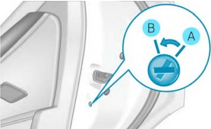
Figure 1. In the left rear door: Child safety lock A is off, and child safety lock B is on.
