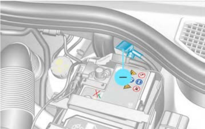
Figure 1. Schematic diagram of jumper cable connection
