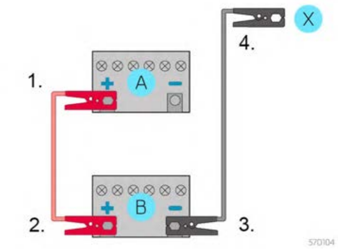
Figure 1. Schematic diagram of jumper cable connection
