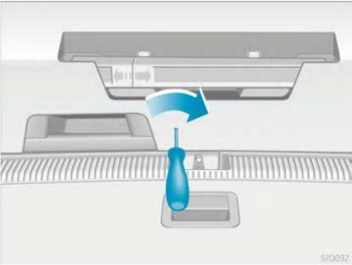
Figure 1: Emergency unlocking device for the trunk lid
